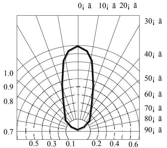
RADIATION DIAGRAM
